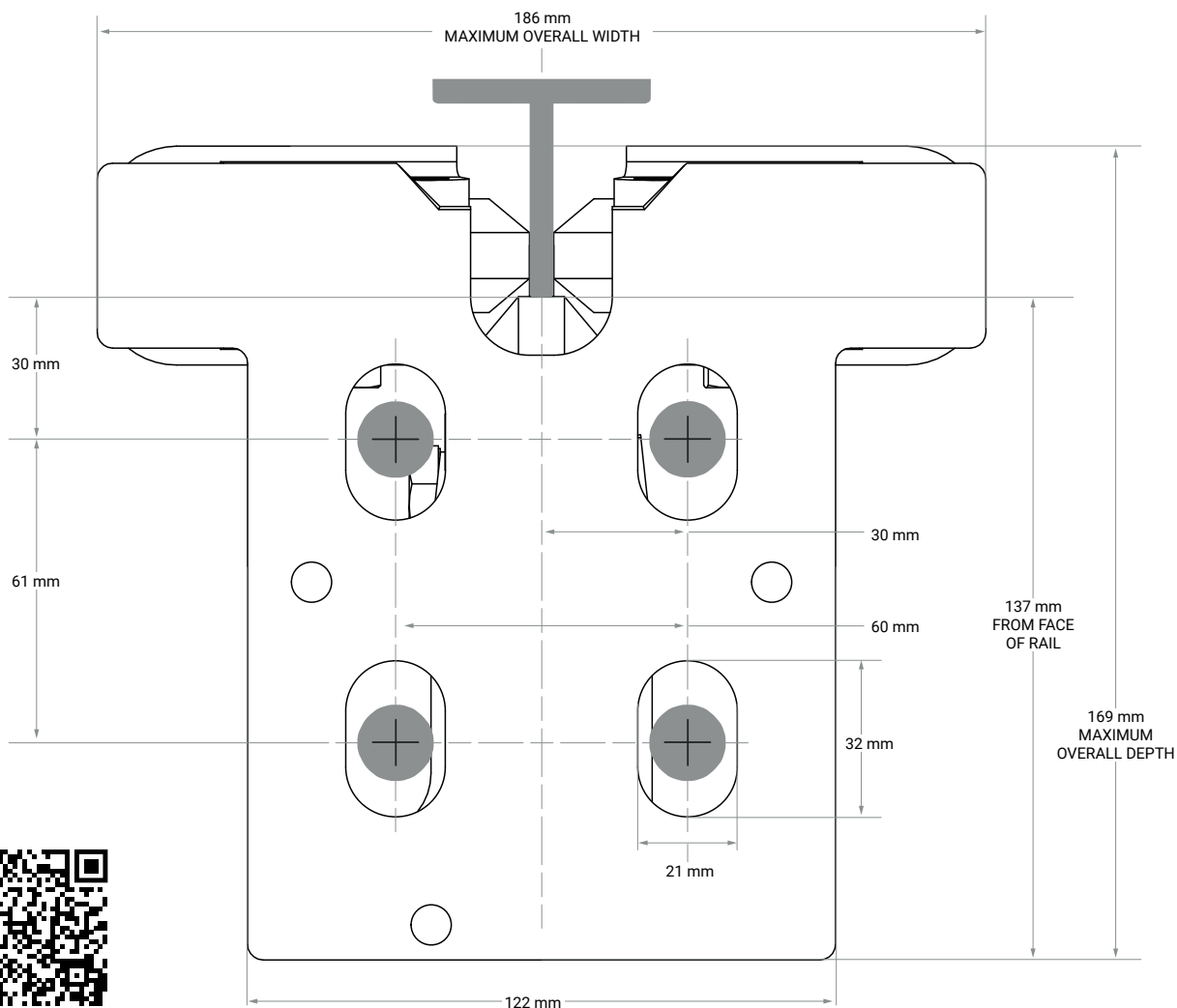
EH211XX Bolt Pattern
