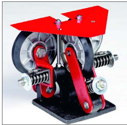
Model B Roller Guide with cover guard
